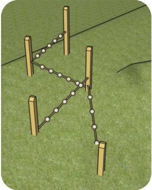
4. TimberForm Rope & Ball Embankment Custom Douglas fir wooden posts
